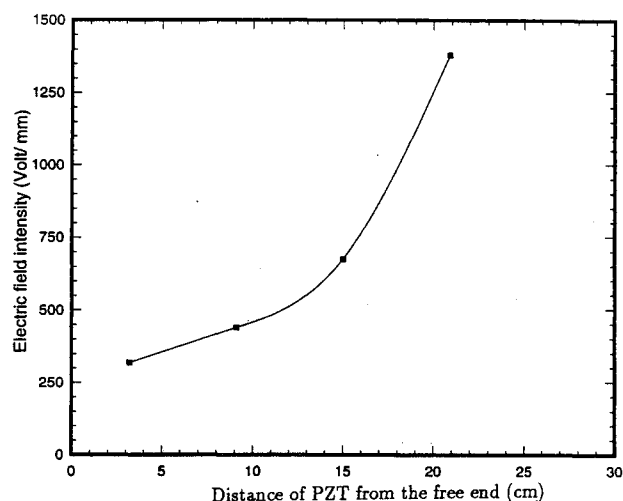
Fig. 6 Electric field intensity required to suppress the tip deflection of a cantilever plate vs the distance of PZTs from the free end.
